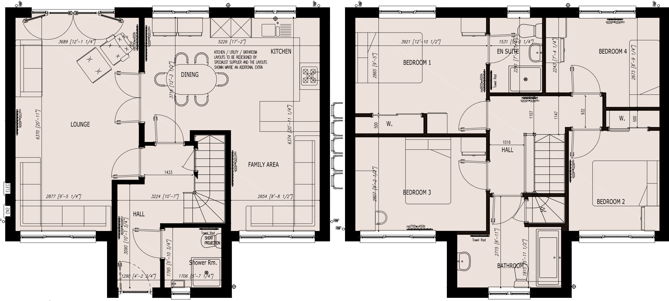
Gross Internal Floor Area including garage 126.6m 2
